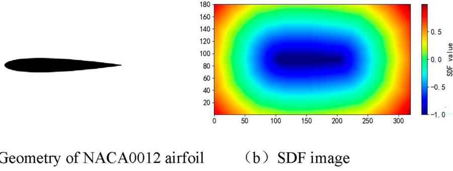
Figure 6. Geometry of airfoil and its SDF image.
